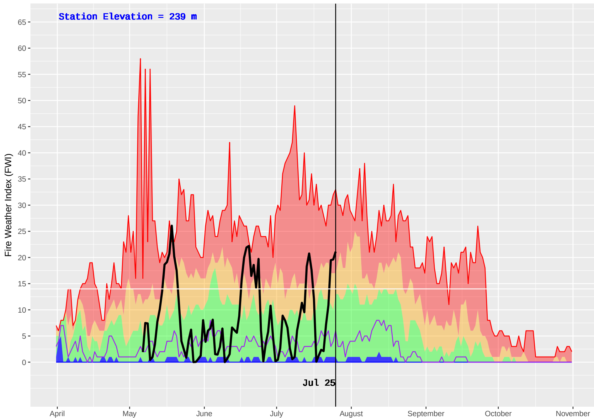
ROSSWOOD (105) : Historical (1970–2016) and Current (2018) Noon Fire Weather Index (FWI)
