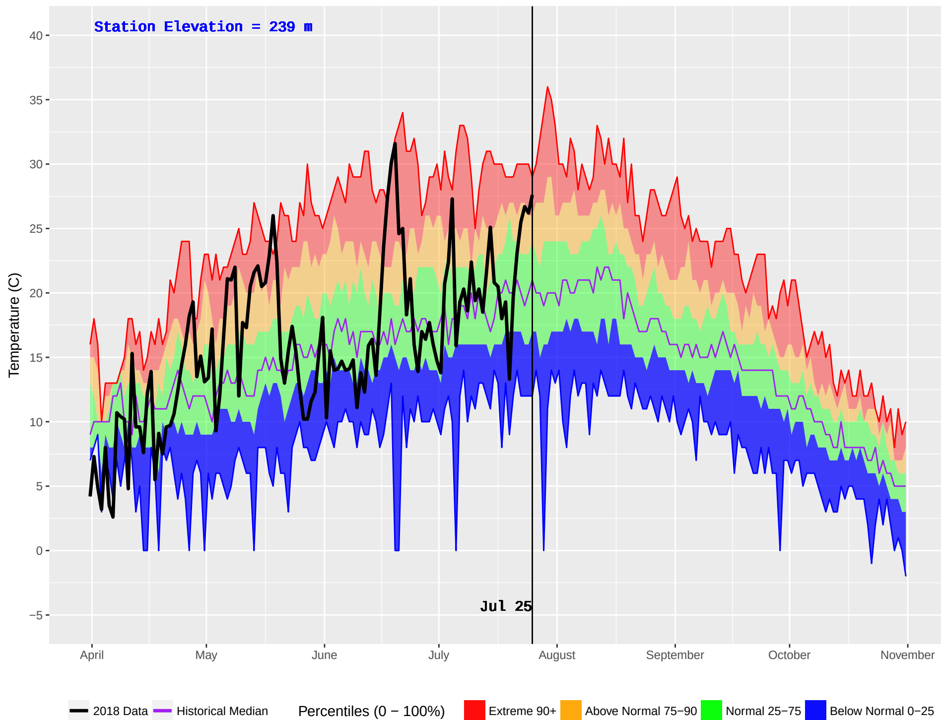
ROSSWOOD (105) : Historical (1970–2016) and Current (2018) Noon Temperature
